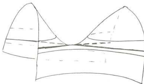
FIGURE 6. le col z = t_0 + x^2 - y^2
