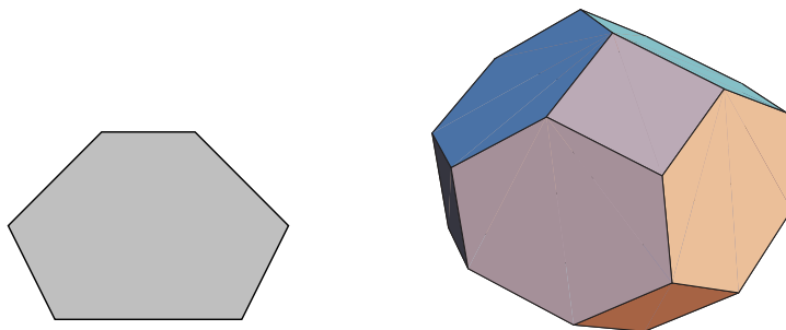
FIGURE 4. Diagonales des matrices n \times n hermitiennes, cas n = 3 et n = 4
